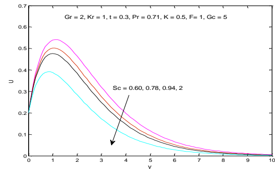
Figure (7): Velocity profiles for different values of Sc
