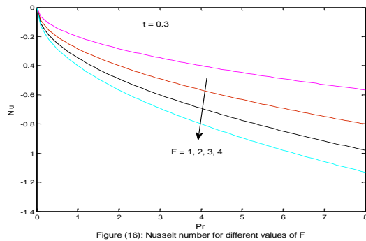
Figure (16): Nusselt number for different values of F
