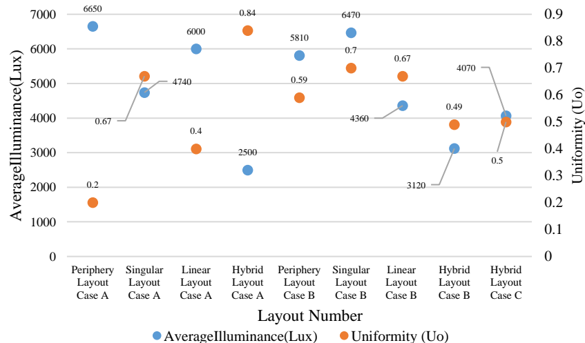
Fig. 8. Illuminance (Lux) index results for nine residential complexes.
