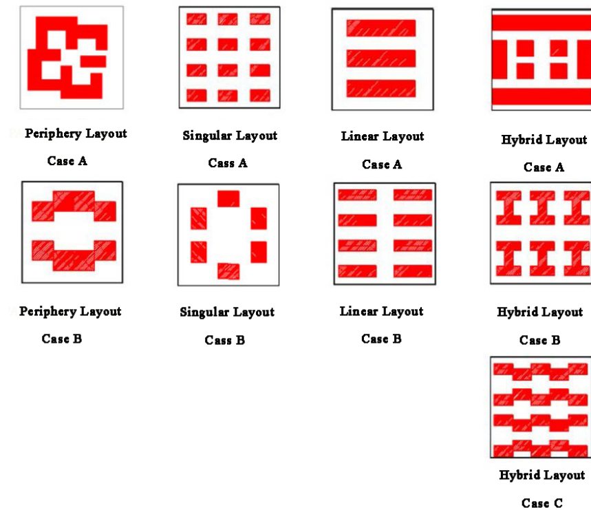
Fig. 2. The normalized layouts extracted of residential complex.
