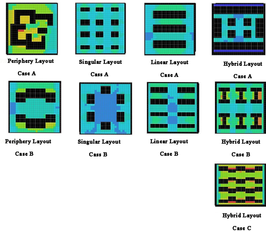
Fig. 6. The Visual Mean Depth index results for nine residential complex layouts.
